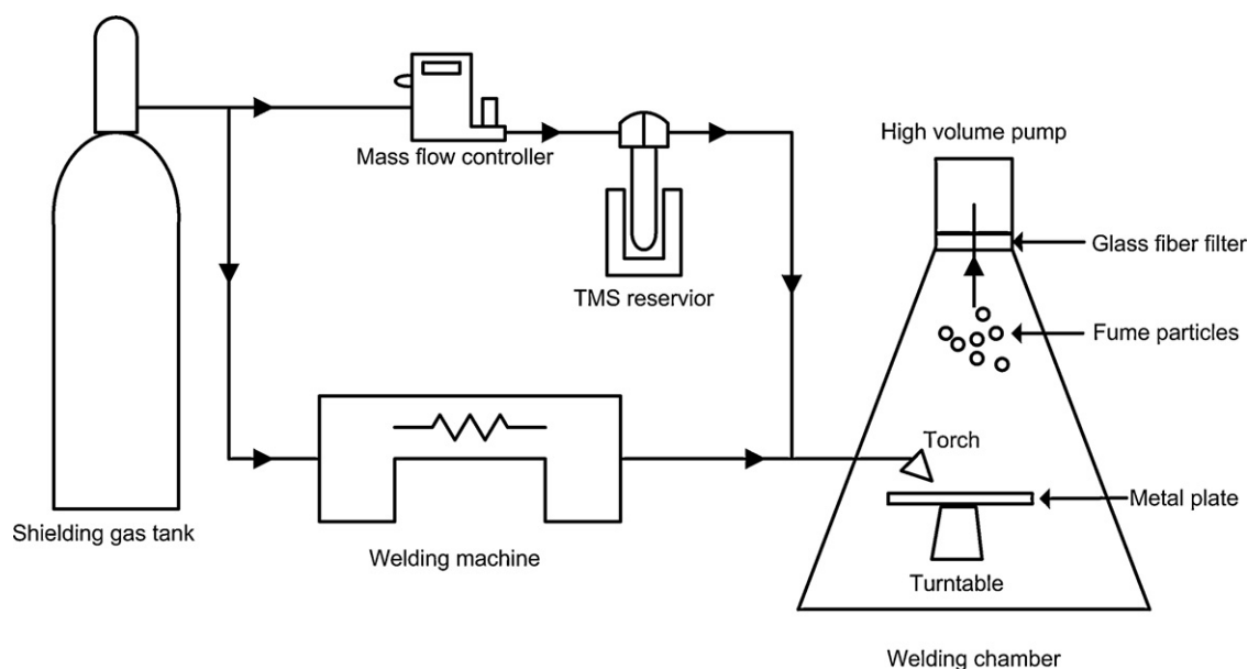
Fig. 1. Schematic diagram for the sampling system.
