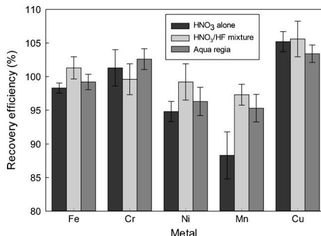
Fig. 2. Recovery efficiencies for Fe, Cr, Ni, Mn, Cu by different digestion acid mixtures.
